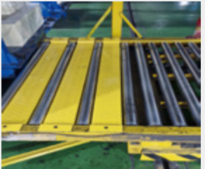
Installation of a Footstep Platform to Prevent Foot Entrapment Between Cart Rollers
